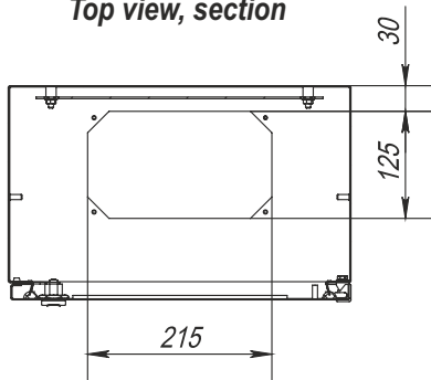
Mounting plate
