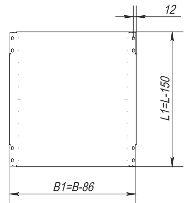
Mounting plate
