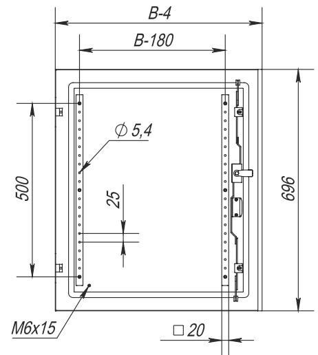
Door, view from the inside
