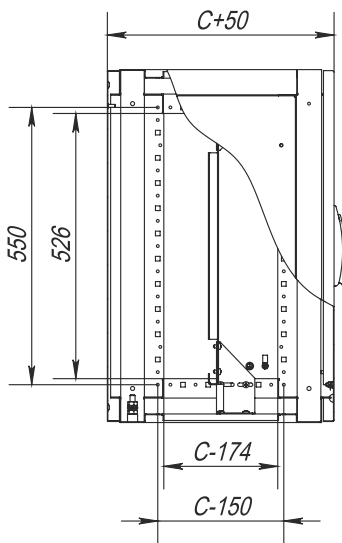
Top view, section
