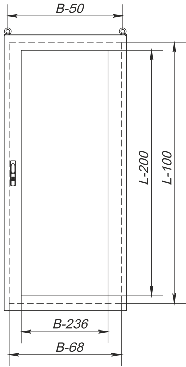
Mounting plate
