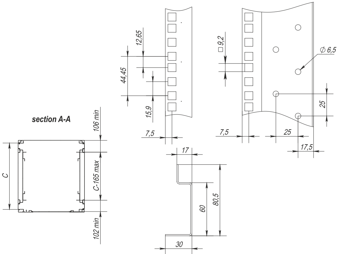
Mounting profil
